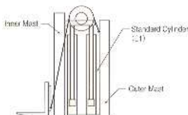
2stage Standard Mast
