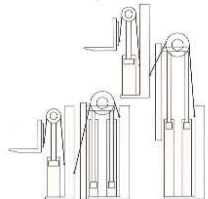
3stage Full Free Mast
